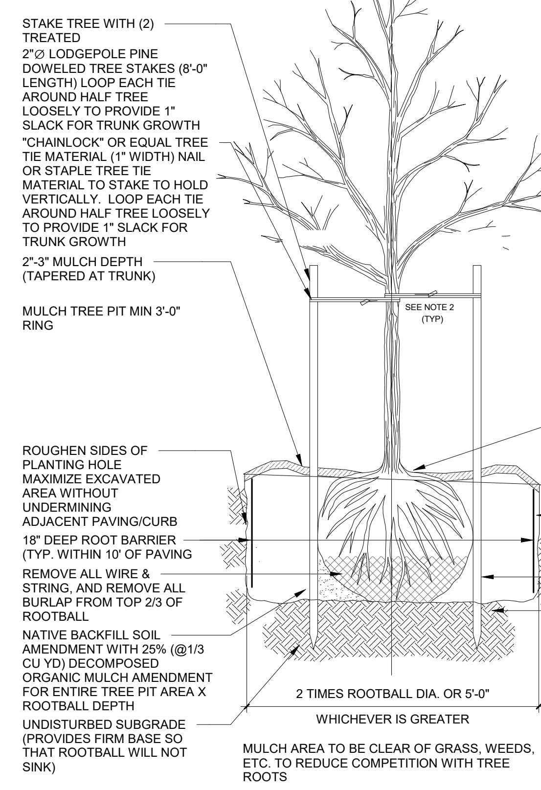
DECIDUOUS TREE PLANTING DETAIL
