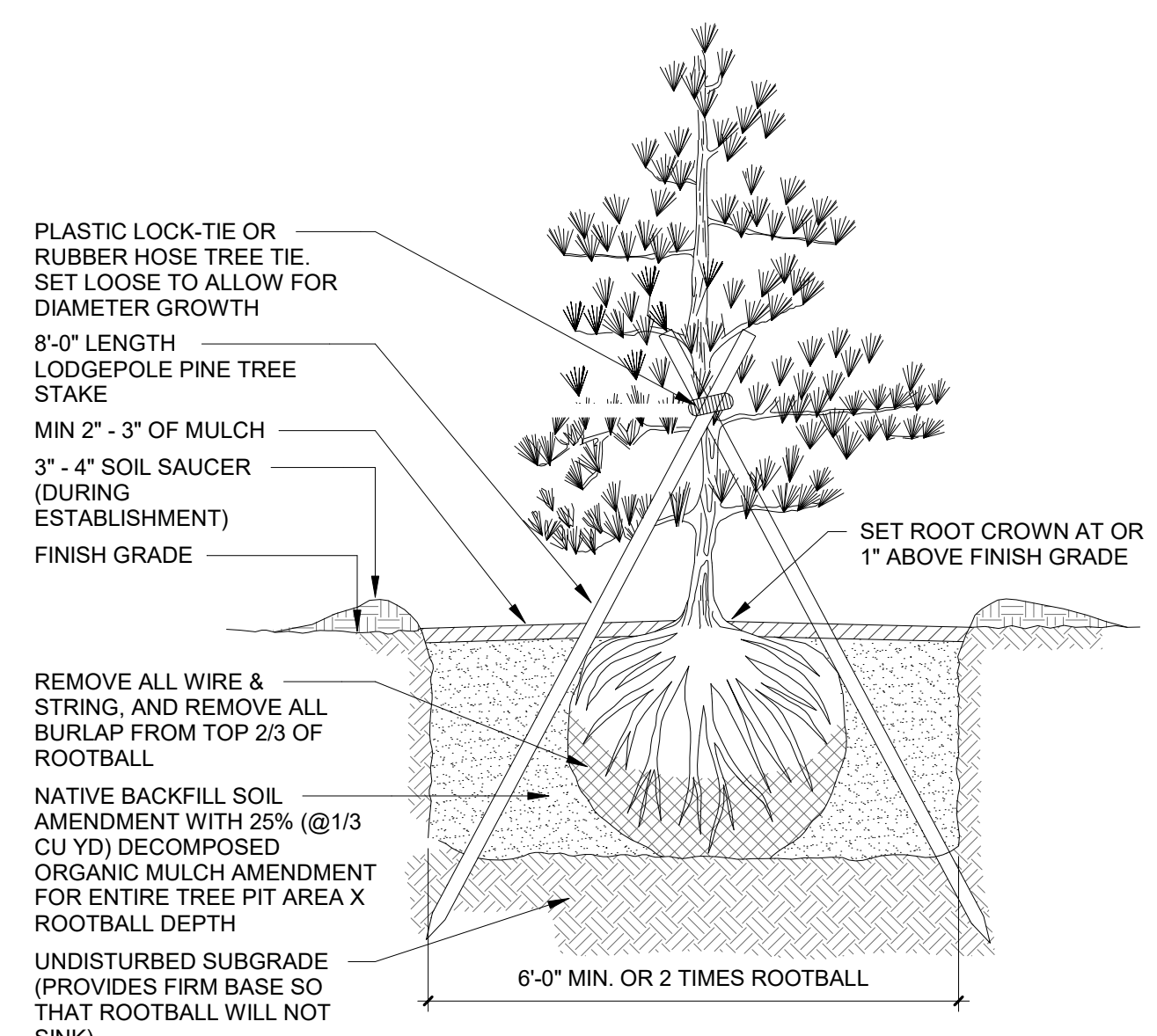
EVERGREEN PLANTING DETAIL
