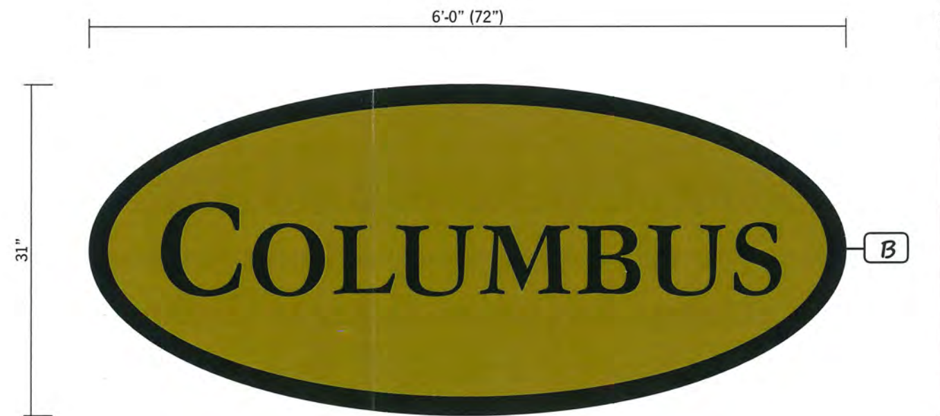
2 FLAT CUT OUT ALUMINUM PLATE LETTERS SCALE: 1"=1'-0"
